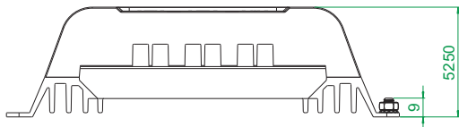
MT1050/1550-EU
