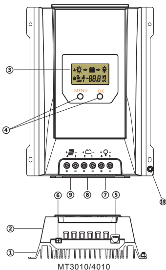
MT3010/4010
