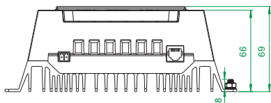
MT3010/4010
